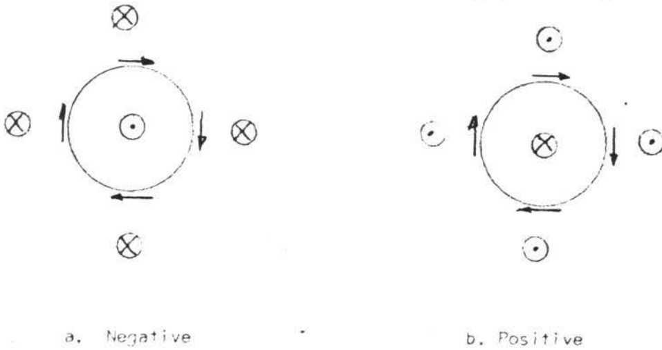
FIGURE 1 CHARGES
