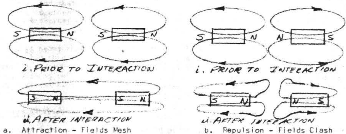
FIGURE 8 MAGNET INTERACTION
