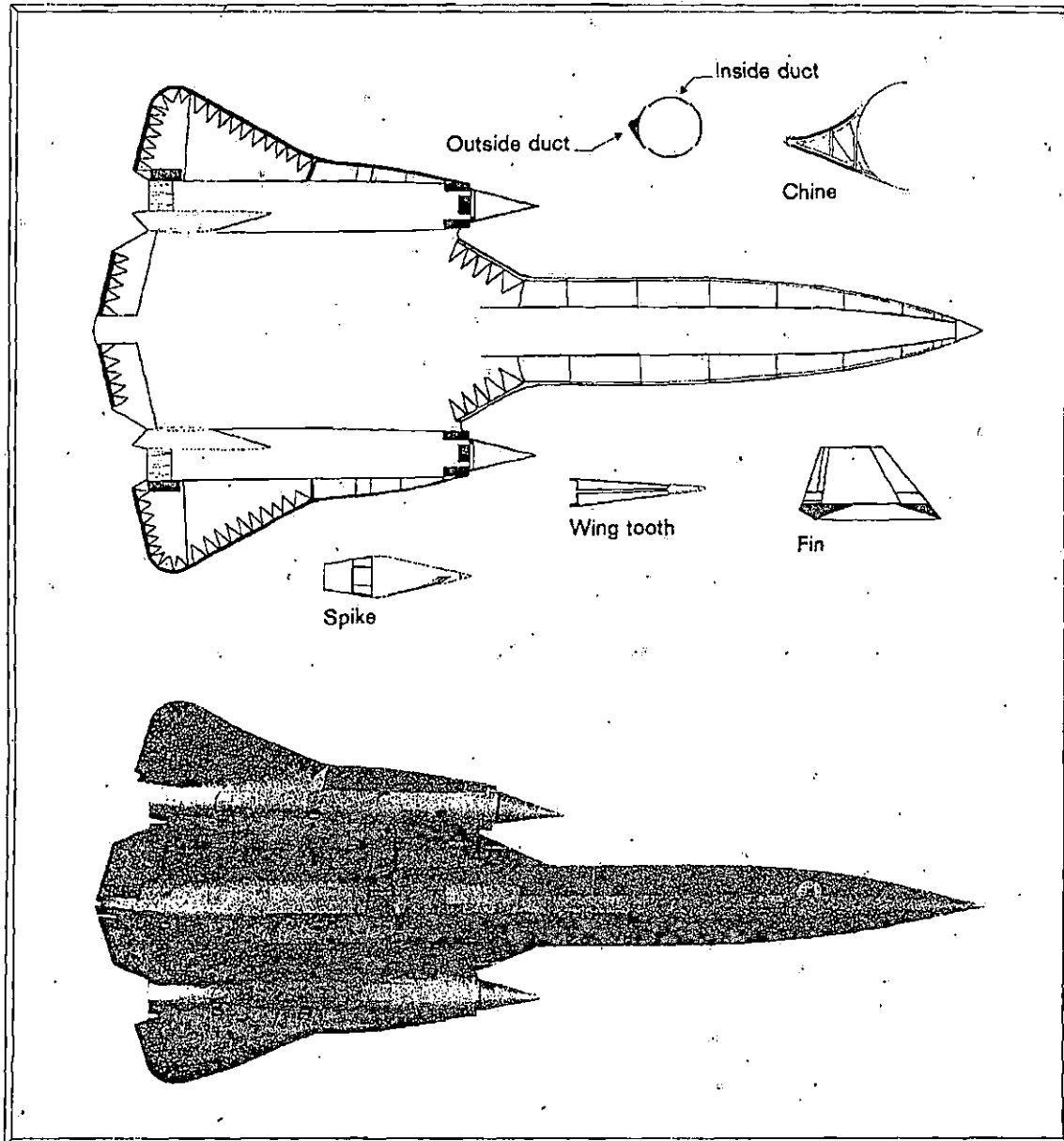
Antiradar features of the A-12
