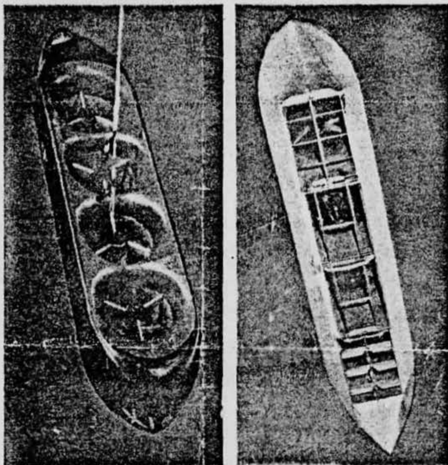
AIRCRAFT'S POWER PLANT is set of fans which draw air through top of model ( left ), expel it past louvers in its belly ( right ). When louvers tilt backward, plane goes forward. When they tilt forward, plane goes backward; when open, plane hovers.
