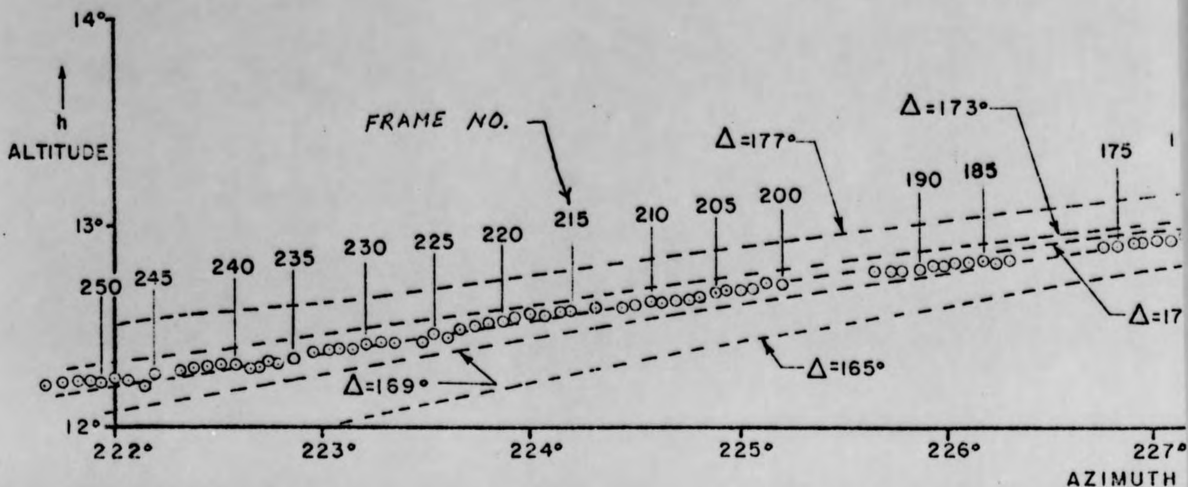
FIGURE 51 SEPARATION DISTANCE
